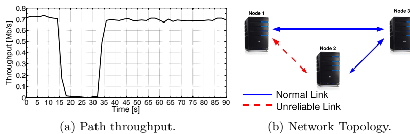
Fig. 3: Testing path reconfiguration delay by simulating a link failure.
