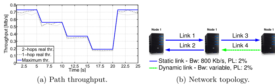
Fig. 2: Controlling a 2-hops path throughput by dynamically reconfiguring a wireless link's parameter (bandwidth).
