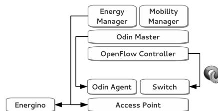
Fig. 1. System architecture. The Odin Master speaks OpenFlow to the switches and uses a custom protocol to communicate with the Odin Agents. The Energy Manager uses a custom protocol to communicate with the APs and with Energino .
