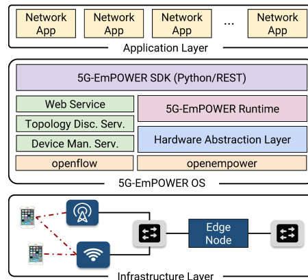
Fig. 4. The 5G-EmPOWER MEC-OS System Architecture.
