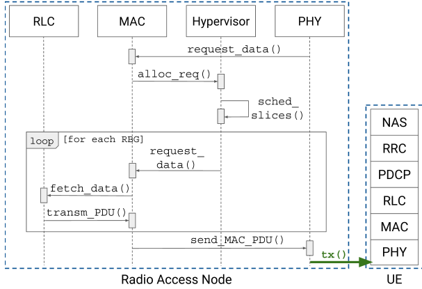
Fig. 7. Resource allocation procedure followed by the RAN slicing solution.
